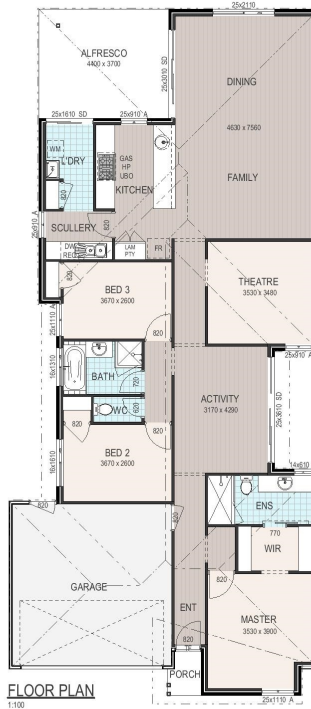
FLOOR PLAN 1:100
